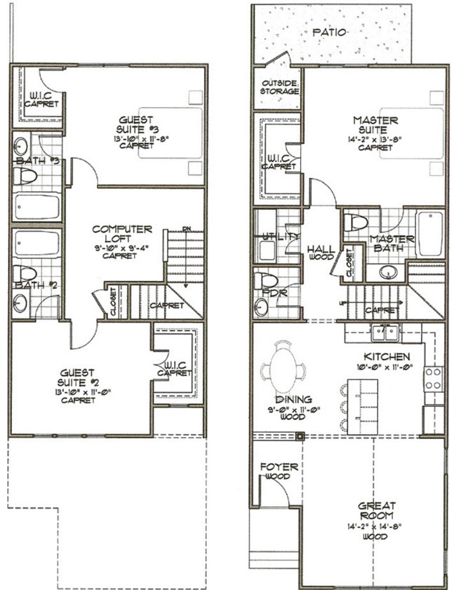
TWO STORY 3 BED 3 1/2 BATH 1700 TOTAL HEATED SQUARE FEET
